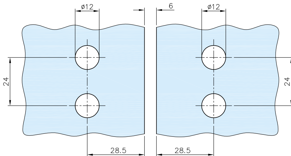
glass cutout
